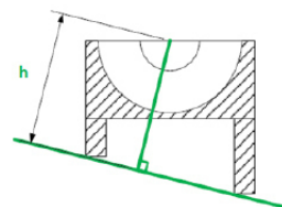
h ≥ 100mm must be respected for at least one cross section of the sump perpendicular to the crankshaft centreline
